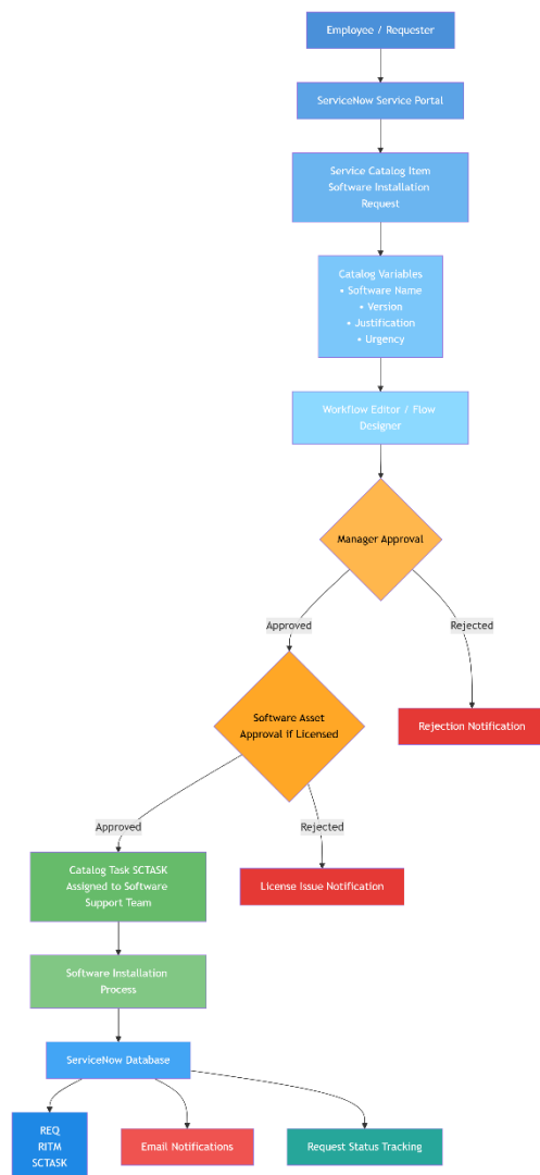
Figure 1: Architecture and data flow of the Software installation Request Automation
